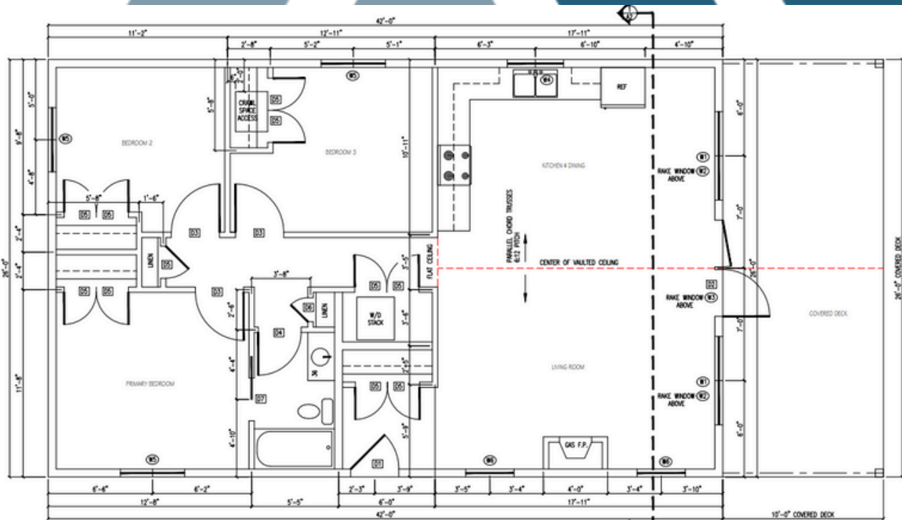
MAIN FLOOR PLAN - NO BASEMENT SCALE: 1/8" = 1'-0" (1092 SQ. FT.)
