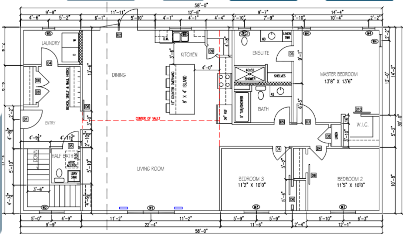
MAIN FLOOR PLAN SCALE: 1/8" = 1'-0" 1740 SQ. FT.
